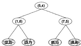
FIGURE 8.11: The initial set of 2D data.
