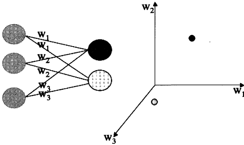
FIGURE 4.1: The position of two neurons in weight space. The labels on the network refer to the dimension in which that weight is plotted, not its value. Note that there is no bias node.
