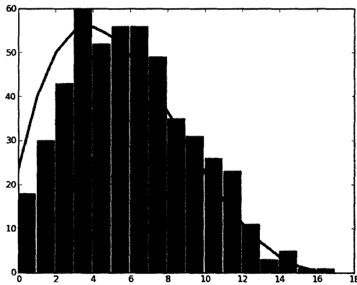
FIGURE 14.8: The Gibbs sampler output for the beta-binomial distribution.
