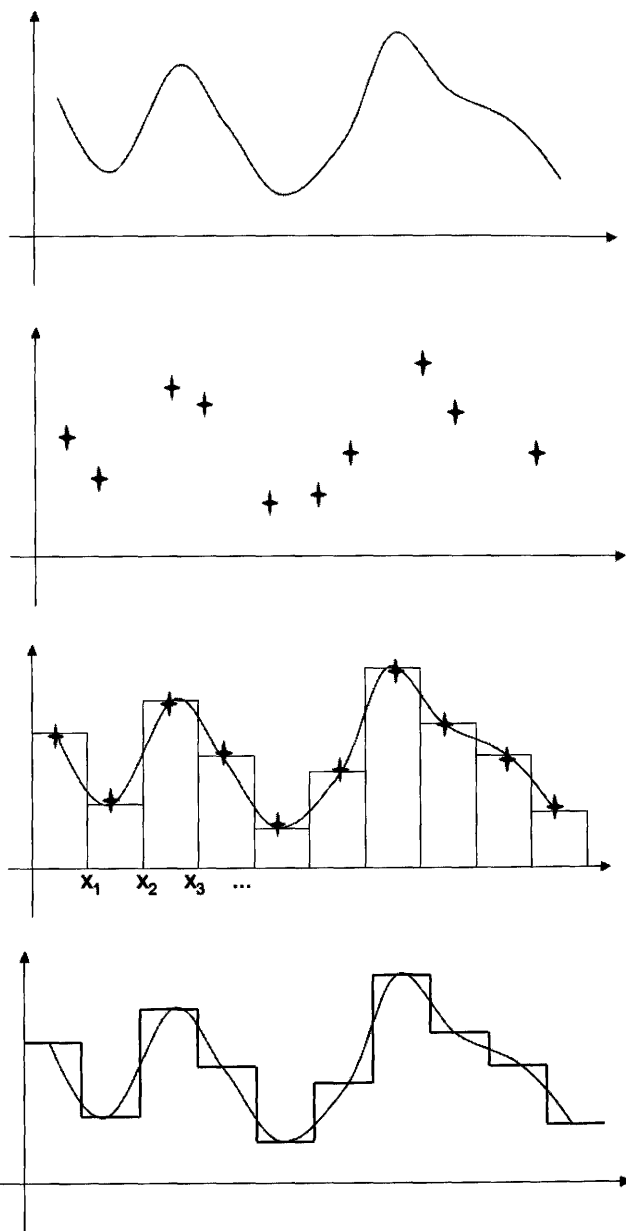
FIGURE 4.9: Top: Curve showing a function. Second: A set of datapoints from the curve. Third: Putting a straight horizontal line through each point creates a histogram that describes an approximation to the curve. Bottom: That approximation.
