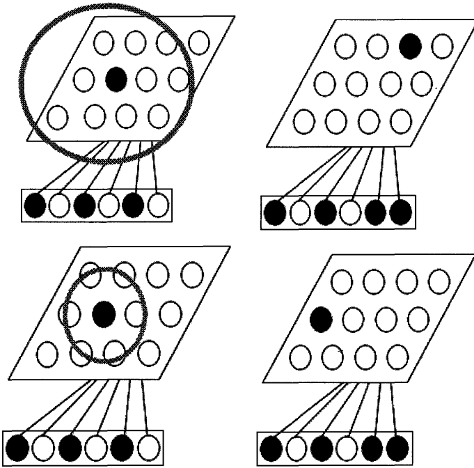
FIGURE 9.9: Top: Initially, similar input vectors excite neurons that are far apart, so that the neighbourhood (shown as a circle) needs to be large. Bottom: Later on during training the neighbourhood can be smaller, because similar input vectors excite neurons that are close together.
