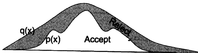
FIGURE 14.2: The proposal distribution method.
