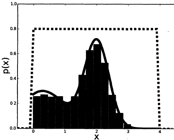
FIGURE 14.4: The histogram shows samples created using sampling-importance-resampling from a mixture of two Gaussians (given by the solid line) as sampled from the uniform box shown as a dotted line.
