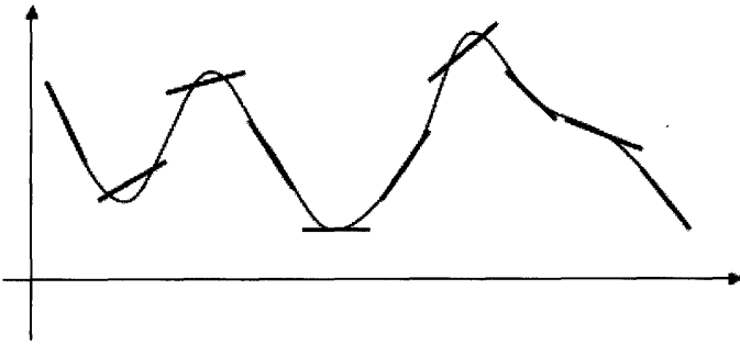
FIGURE 4.10: Representing the points by straight lines that aren't necessarily horizontal (so that their first derivative matches at the point) gives a better approximation.
