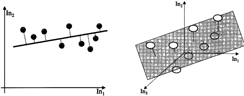
FIGURE 2.12: Linear regression in two and three dimensions.
