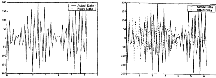
FIGURE 11.4: Using Levenberg-Marquardt for least-squares data fitting of data from Equation (11.18). The example on the left converges to the correct solution, while the one on the right, which still starts from a point close to the correct solution, fails to find it, resulting in significantly different output.
