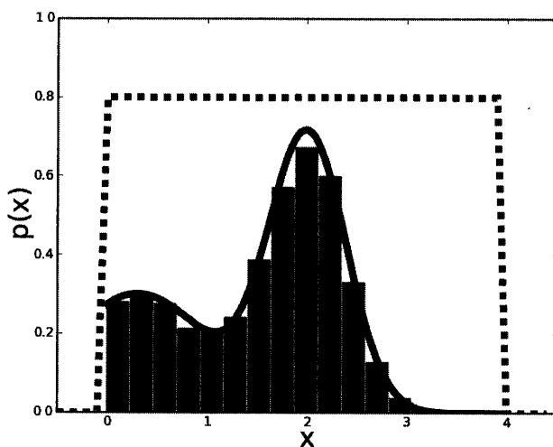
FIGURE 14.3: The histogram shows samples of a mixture of two Gaussians (given by the solid line) as sampled from the uniform box shown as a dotted line by using rejection sampling.
