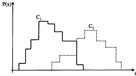
FIGURE 8.1: A histogram of feature values ( x ) against their probability for two classes.
