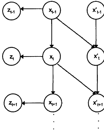
FIGURE 15.10: A representation of the Kalman filter as a graphical model.
