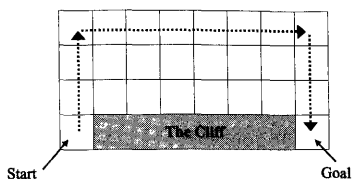
FIGURE 13.8: The sarsa solution is far from optimal, but it is safe.
