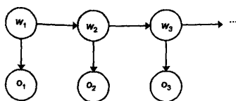
FIGURE 15.6: The Hidden Markov Model is an example of a dynamic Bayesian network. The figure shows the first three states and the related observations unrolled as time progresses.
