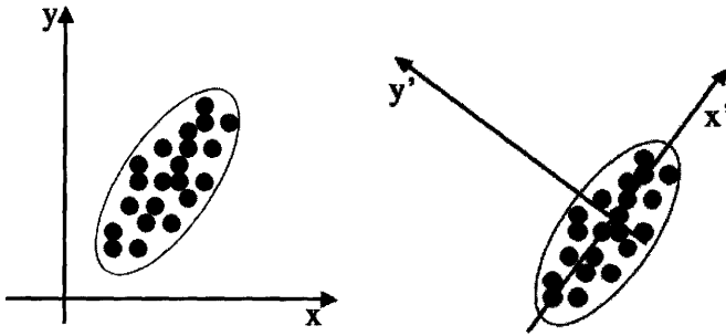
FIGURE 10.6: Two different sets of coordinate axes. The second consists of a rotation and translation of the first and was found using Principal Components Analysis.
