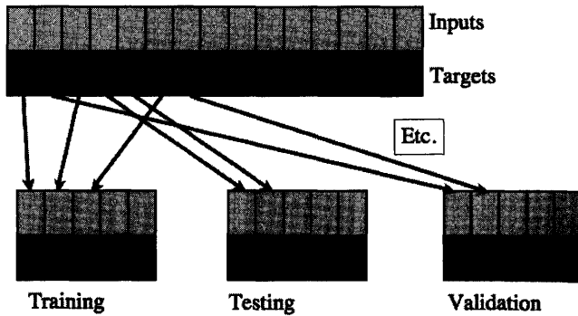
FIGURE 3.12: The dataset is split into different sets, some for training, some for validation, and some for testing.
