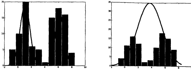
FIGURE 8.7: Histograms of training data from a mixture of two Gaussians and two fitted models, shown as the line plot. The model shown on the left fits well, but the one on the right produces two Gaussians right on top of each other that do not fit the data well.
