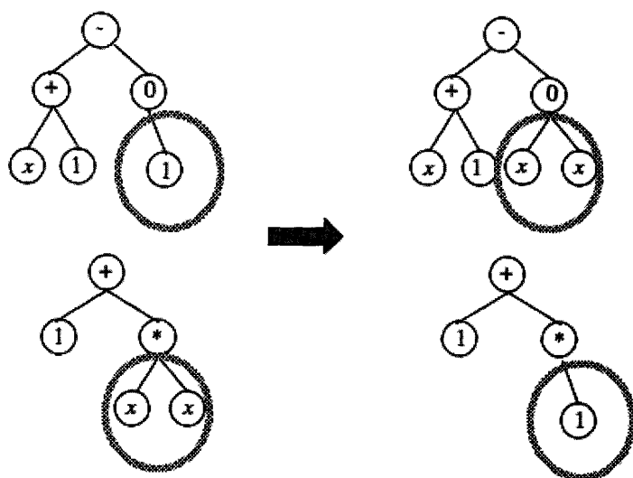
FIGURE 12.14: Example of a crossover in genetic programming.
