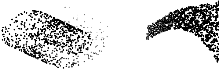
FIGURE 10.13: A common example used to demonstrate LLE is the swissroll dataset shown on the left. To produce a useful 2D representation of this data requires unrolling the data, which the LLE does successfully, as is shown on the right. The shades are used to identify neighbouring points, and do not have any other purpose.
