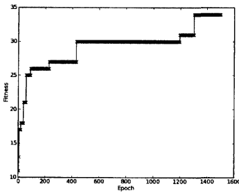
FIGURE 12.11: Evolution of a solution to the four peaks problem. The solution never reaches the bonus score in the fitness function.
