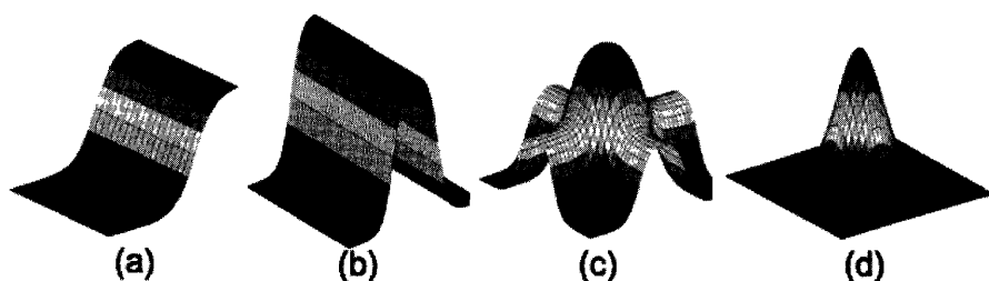
FIGURE 3.9: The learning of the MLP can be shown as (a) the output of a single sigmoidal neuron can be added to others (b), including reversed ones, to get a hill shape. Adding another hill at 90^\circ produces (c) a bump, which can be sharpened (d) to any extent we want, with the bumps added together in the output layer. Thus the MLP learns a local representation of individual inputs.
