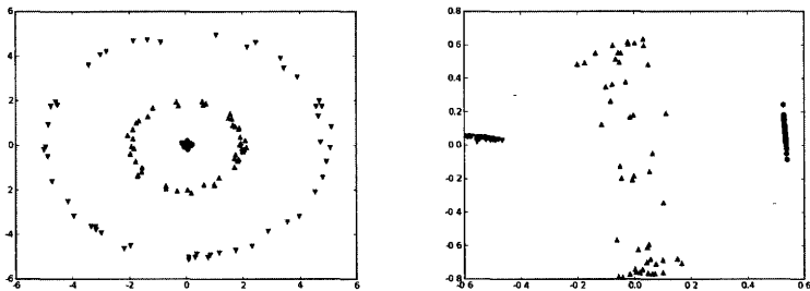
FIGURE 10.10: A very definitely non-linear dataset consisting of three concentric circles, and the kernel PCA mapping of the data, which requires only one component to separate the data.
