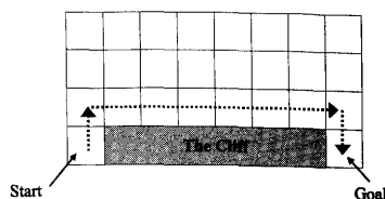
FIGURE 13.9: The Q-learning solution is optimal, but occasionally the random search will tip it over the cliff.
