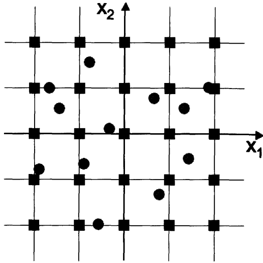
FIGURE 4.15: In 2D the knotpoints (black squares) can be used to interpolate other points (grey circles) in each dimension individually.
