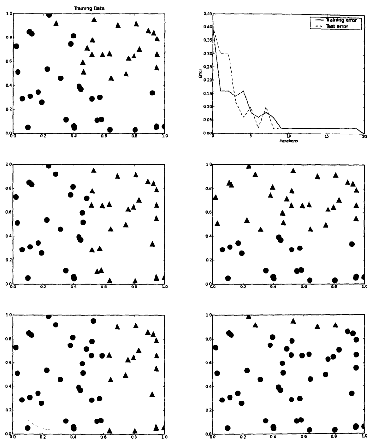
FIGURE 7.4: Top: the training data and the error curve. Middle and bottom: The first few iterations of the classifier; each plot shows the output of one of the weak classifiers that are boosted by the algorithm.
