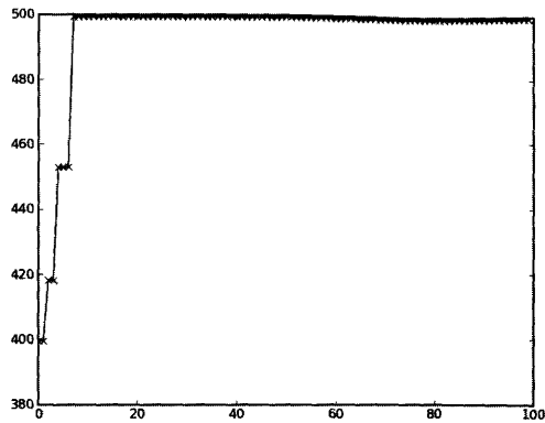
FIGURE 12.10: Evolution of the solution to the knapsack problem. The GA finds a very good solution to this simple problem within a few iterations, but never finds the optimal solution.
