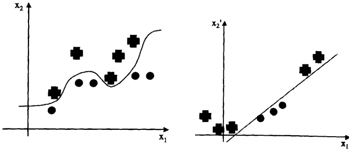
FIGURE 5.4: By modifying the features we hope to find spaces where the data are linearly separable.
