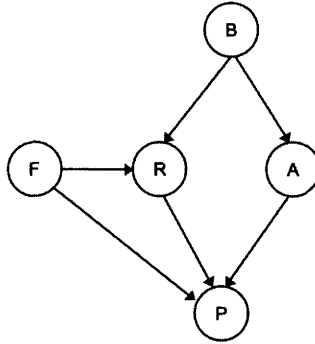
FIGURE 15.3: Adding just one extra node ('F', information about whether or not this is your final year) makes the conditional probability tables significantly more complicated.
