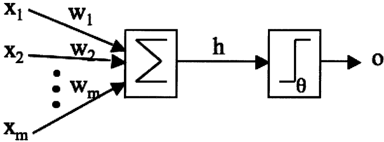
FIGURE 1.6: A picture of McCulloch and Pitts's mathematical model of a neuron. The inputs x_i are multiplied by the weights w_i , and the neurons sum their values. If this sum is greater than the threshold \theta then the neuron fires, otherwise it does not.
