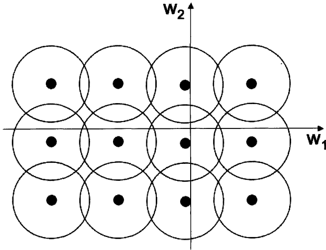
FIGURE 4.5: We can space out RBF nodes to cover the whole of space by continuing this pattern everywhere, so that the network acts as a universal approximator, since there is an output for every possible input.
