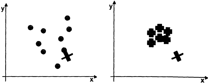
FIGURE 8.4: Two different datasets and a testpoint.
