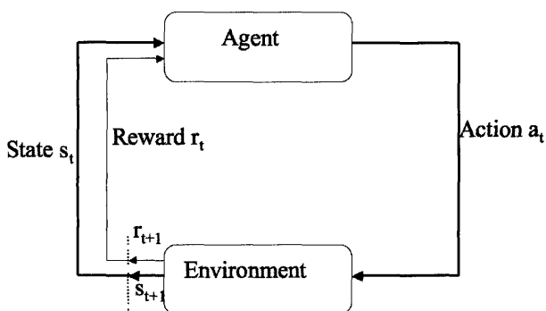
FIGURE 13.2: The reinforcement learning cycle: the learning agent performs action a_t in state s_t and receives reward r_{t+1} from the environment, ending up in state s_{t+1} .
