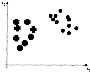
FIGURE 10.2: A set of datapoints in two dimensions, with two classes.
