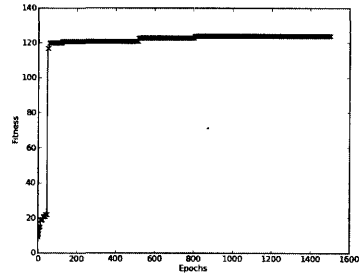
FIGURE 12.12: Another solution to the four peaks problem. This solution does reach the bonus score, but does not get the global maximum.
