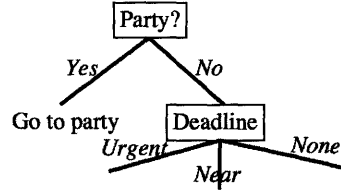
FIGURE 6.7: The tree after another step.
