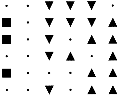
FIGURE 9.13: Plot showing which nodes are the best match according to class, with the three shapes corresponding to three different classes in the iris dataset. The small dots represent nodes that did not fire.
