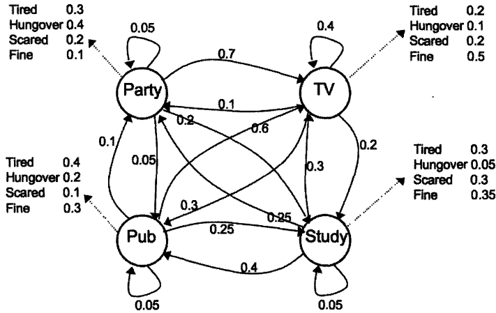
FIGURE 15.7: The example HMM with transition and observation probabilities shown.
