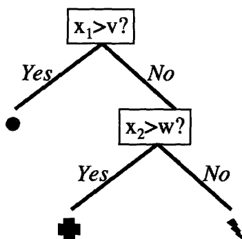
FIGURE 6.5: The final tree created by the splits in Figure 6.4.
