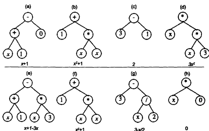
FIGURE 12.15: Top : Four arithmetical trees. Bottom : Example developments of the four trees: (e) and (h) are a possible crossover of (a) and (d), (f) is a copy of (b), and (g) is a mutation of (c).
