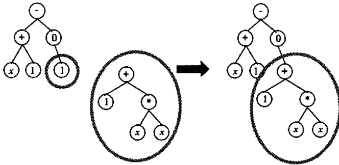
FIGURE 12.13: Example of a mutation in genetic programming.
