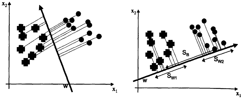
FIGURE 10.4: Two different possible projection lines. The one on the left fails to separate the classes.
