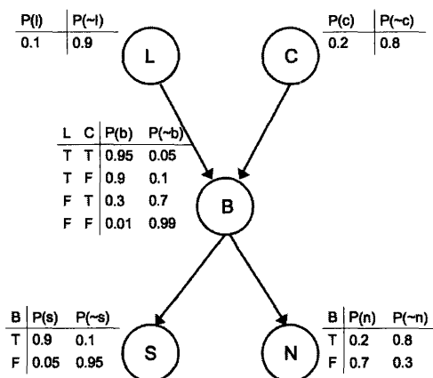
FIGURE 15.14: The Bayesian Network example for Problem 15.1.
