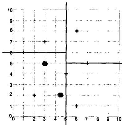
FIGURE 8.14: Two testpoints for the example KD-tree.
