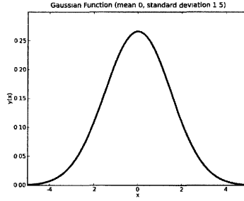
FIGURE 8.5: Plot of the one-dimensional Gaussian curve.
