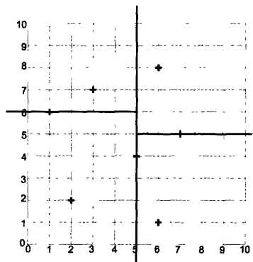
FIGURE 8.12: The splits and leaf points found by the KD-tree.
