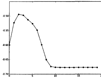
FIGURE 8.8: Plot of the log likelihood changing as the Gaussian Mixture Model EM algorithm learns to fit the two Gaussians shown on the left of Figure 8.7.
