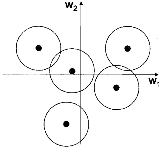
FIGURE 4.3: The effect of radial basis functions in weight space. The points show the position of the RBF in weight space, while the circle around each point shows the receptive field of the node. In higher dimensions these circles become hyperspheres.
