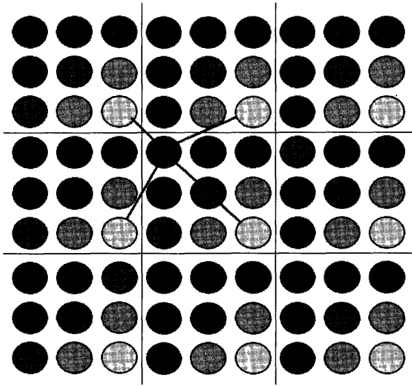
FIGURE 9.11: One way to compute distances between points without any boundary on the map is to imagine copies of the entire map being placed around the original, and picking the shortest of the distances between a node and any of the copies of the other node.
