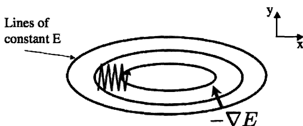
FIGURE 3.7: In 2D, downhill means at right angles to the lines of constant contour. Imagine walking down a hill with your eyes closed. If you find a direction that stays flat, then at right angles to that there may well be uphill or downhill. However, this is not the direction that takes you directly towards the local minimum.
