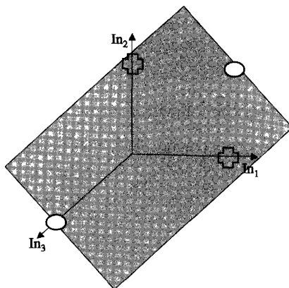
FIGURE 2.9: A decision boundary (the shaded plane) solving the XOR problem in 3D with the crosses below the surface and the circles above it.
