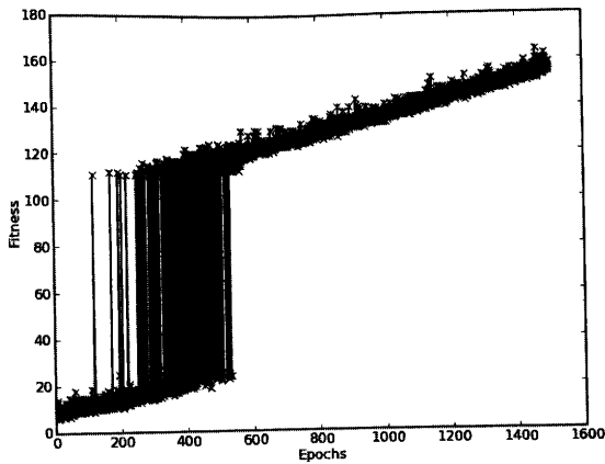
FIGURE 12.16: The evolution of the best fitness using PBIL on the four peaks problem.
