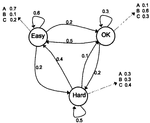
FIGURE 15.15: The Hidden Markov Model example for Problem 15.3.
