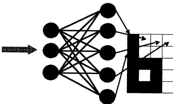
FIGURE 3.22: Schematic showing how the hidden nodes and second layer of weights can be used to regain the compressed images after the network has been trained.
