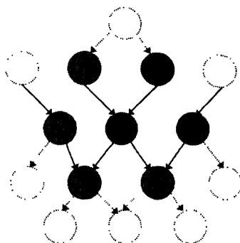
FIGURE 15.4: The Markov blanket of a node is the set of nodes (shaded light grey) that are either parents or children of the node, or other parents of its children (shaded dark grey).
