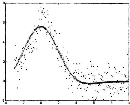
FIGURE 4.13: Using linear least-squares to fit parameters for two Gaussians produces the line from the noisy datapoints plotted as circles.
