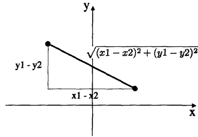
FIGURE 8.15: The Euclidean and city-block distances between two points.
