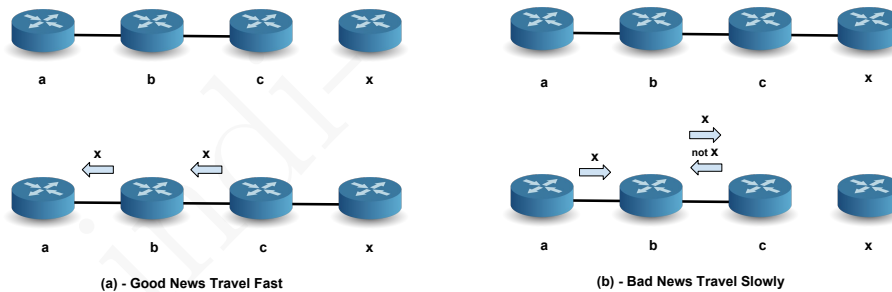
Figura 16.17: Ilustração do fenómeno “as boas notícias correm velozes, mas as más devagar” (“ good news travel fast, while bad news travel slowly ”).
