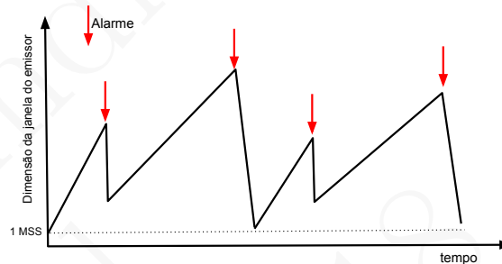
Figura 8.14: Additive increase multiplicative decrease
