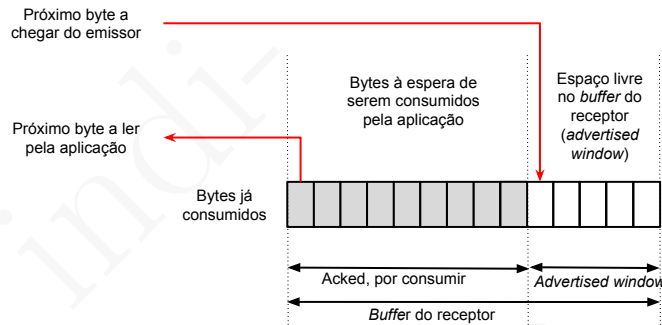
Figura 7.9: Janela de receptor e cálculo do valor de receiver advertised window no TCP
