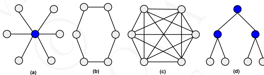
Figura 4.5: Redes (a) estrela ( hub-spoke ), (b) anel ( ring ), (c) malha completa ( full-mesh ), (d) hierárquica ( hierarchical )
