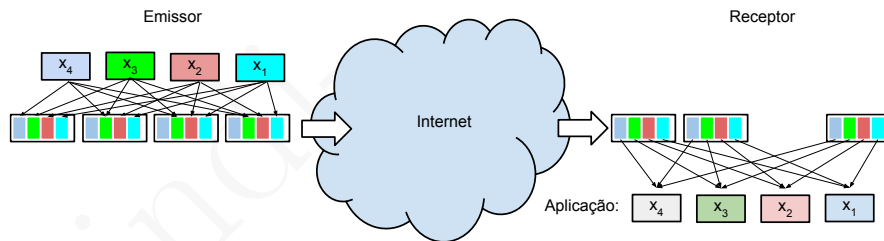
Figura 9.12: FEC – Forward Error Correction com Interleaving de sub-intervalos
