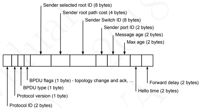
Figura 15.8: STP BPDUs ( Bridge Protocol Data Unit )
