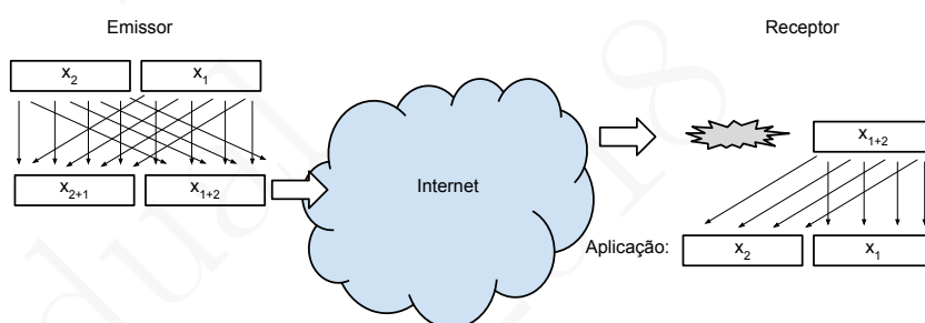
Figura 9.11: Forward Error Correction com interleaving byte a byte
