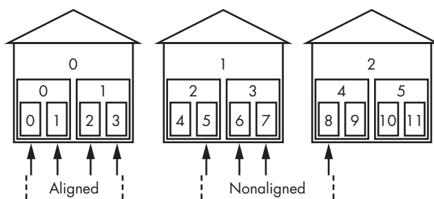
Figure 4-3: Aligned and nonaligned accesses
