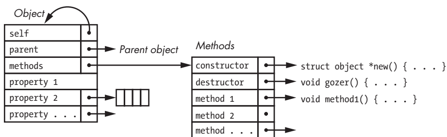
Figure 7-39: Separate method structure
