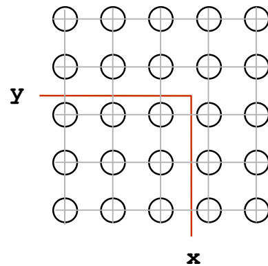
True location
