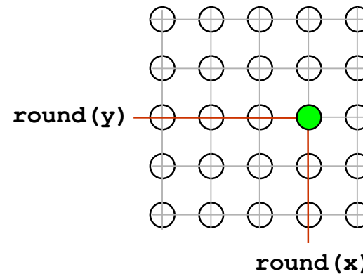
Alias location
