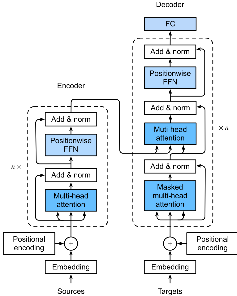
Fig. 10.7.1: The Transformer architecture.
