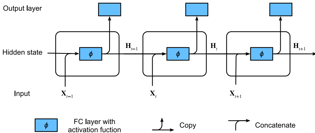
Fig. 8.4.1: An RNN with a hidden state.
