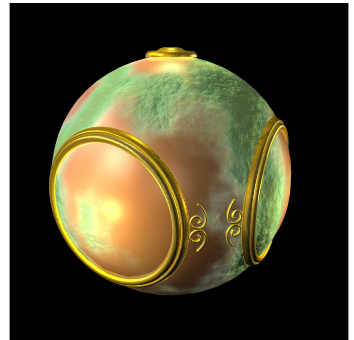
bump mapping
